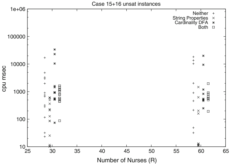
Fig. 10 Runtimes (in milliseconds) of the unsatisfiable instances of NSPLib cases 15 and 16 using neither, either, or both of our methods
