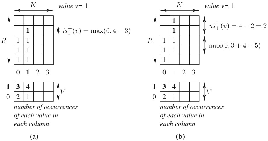
Fig. 3 Lower and upper bounds on the number of stretches starting at a given column. Boldface in the R \times K matrices corresponds to stretches of value 1 starting at column 1 that we are trying to minimise (a) or maximise (b). Boldface in the V \times K matrices corresponds to the occurrence constraints on value v = 1
