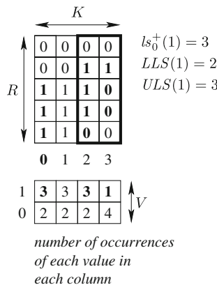
Fig. 4 Minimum number of occurrences of values 0 and 1 in columns 2 and 3 with respect to (a) the minimum number of stretches starting in another column and (b) the minimum and maximum stretch lengths. In the R \times K matrix, boldface in column 0 corresponds to the requirement ls_0^+(1) = 3 , whereas boldface 1s in the box corresponds to the left hand side of (25); boldface 0s correspond to the term ls_0^+(1) ; boldface 1s correspond to the term \sum_{j=2}^3 \#_j^1 . Boldface in the V \times K matrix corresponds to the occurrence constraints on value v = 1
