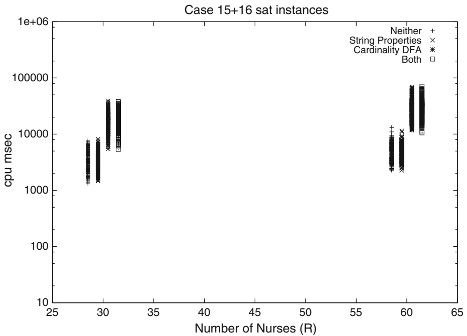
Fig. 9 Runtimes (in milliseconds) of the satisfiable instances of NSPLib cases 15 and 16 using neither, either, or both of our methods
