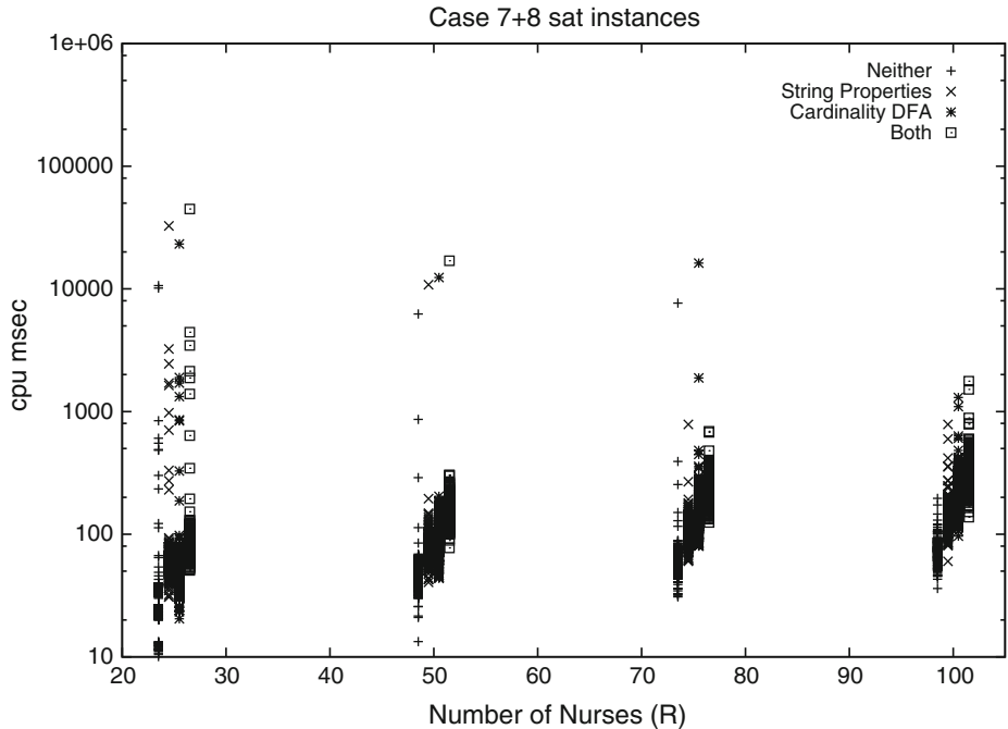
Fig. 7 Runtimes (in milliseconds) of the satisfiable instances of NSPLib cases 7 and 8 using neither, either, or both of our methods
