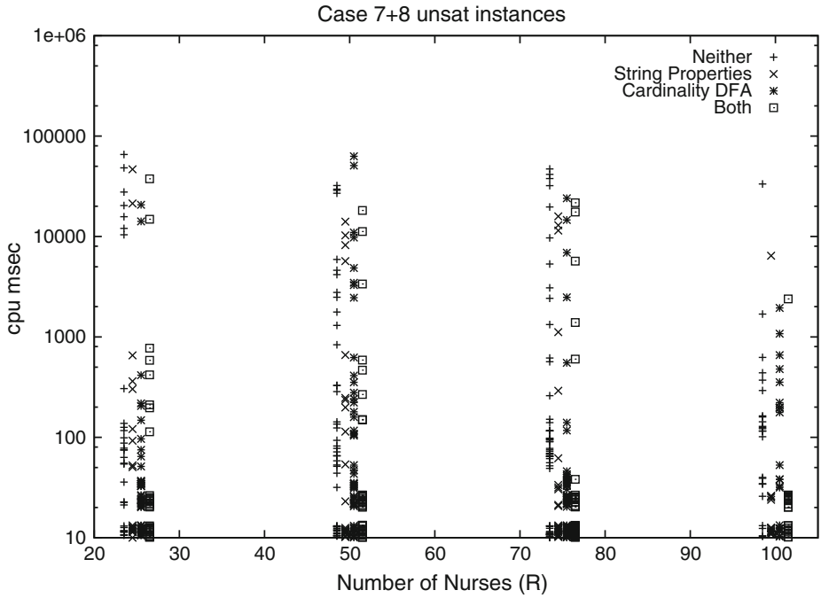
Fig. 8 Runtimes (in milliseconds) of the unsatisfiable instances of NSPLib cases 7 and 8 using neither, either, or both of our methods
