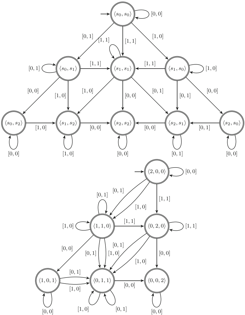
Fig. 6 (Top): vector automaton \overline{C}_2 for the (counter-free version of the) automaton C (with p = 3 states) in Fig. 1 for the global_contiguity constraint and vectors of R = 2 elements over the set \{0, 1\} . (Bottom): cardinality automaton \#(\overline{C}_2) for the automaton C and vectors of R = 2 elements
