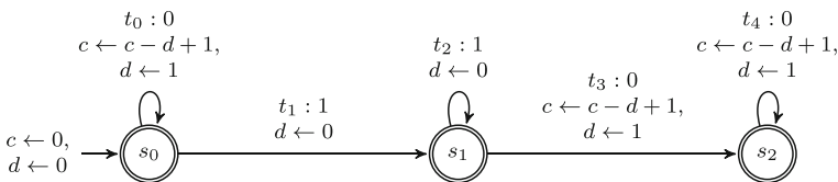
Fig. 1 Automaton \mathcal{C} associated with the global_contiguity constraint, with initial state s_0 , accepting states s_0, s_1, s_2 , and transitions t_0, t_1, t_2, t_3, t_4 labelled by values 0 or 1. The missing transition for value 1 from state s_2 is assumed to go to a dead state. The automaton has been annotated with counters [3]: the final value of counter c is the number of stretches of value 0, whereas d is an auxiliary counter
