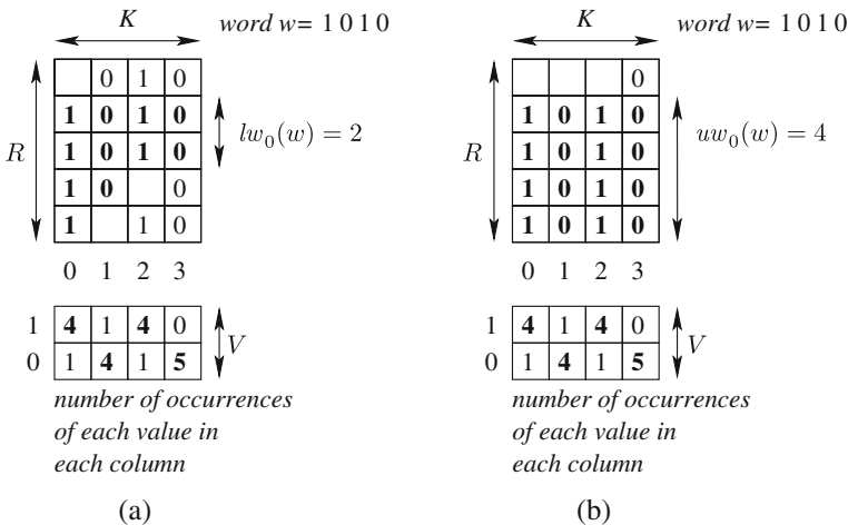
Fig. 2 Lower and upper bounds on the number of words starting at a given column. Boldface in the R \times K matrices corresponds to partial instances of the word w = 1010 for which we try to minimise (a) or maximise (b) the number of occurrences. Boldface in the V \times K matrices corresponds to letters of the word w = 1010
